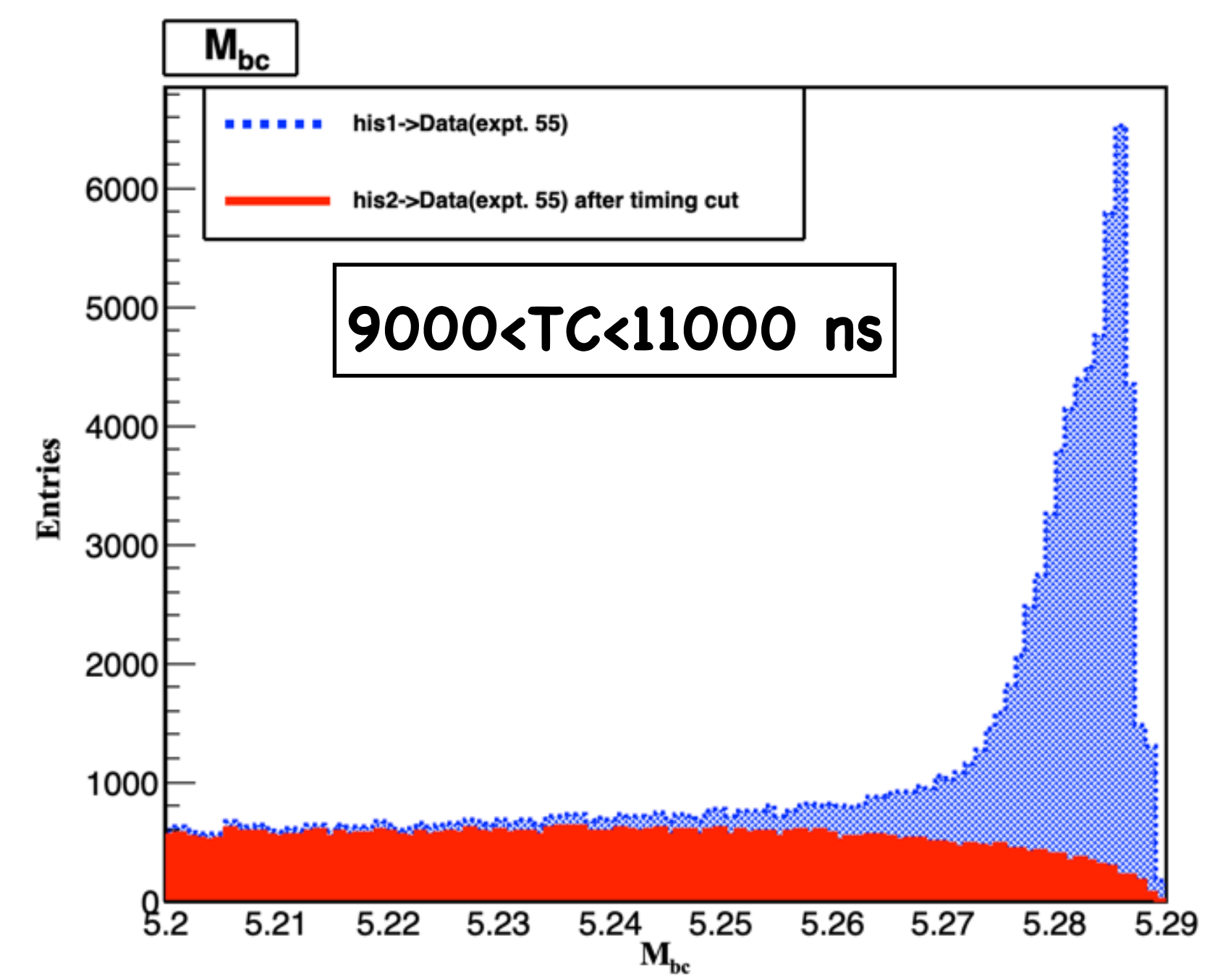
Fig 2: Peaking component rejected after applying the timing cut in real data
