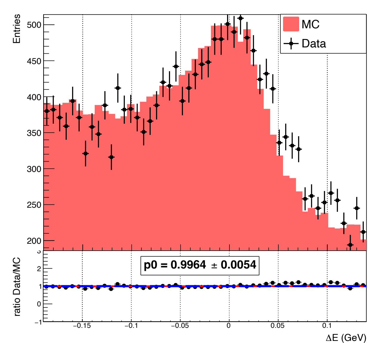
Data-MC comparison for M_{bc} and \Delta E for Belle
