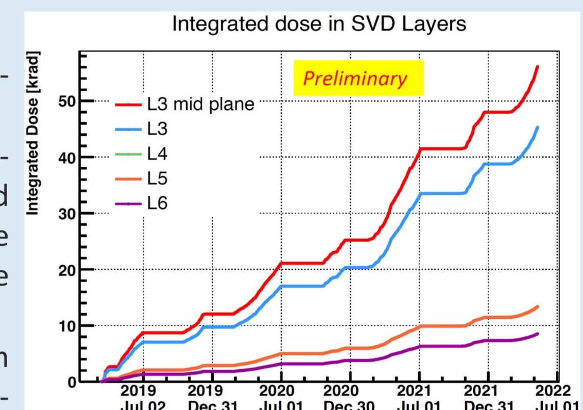
Integrated dose per SVD layer. The dose in layer 4 and 5 is very similar, thus they overlap in this plot.
