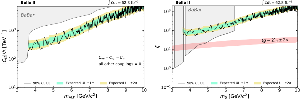
Figure 3. Observed upper limit set by Belle II in the e^+e^- \rightarrow \mu^+\mu^-X, X \rightarrow \tau^+\tau^- search on parameter space for Axion-Like Particles (left) and Dark Scalars (right) [19].
