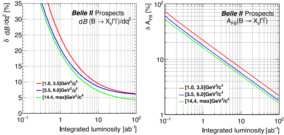
Figure 4: The Belle II sensitivity projection for BF(B \rightarrow X_s \ell^+ \ell^-) (left) and \mathcal{A}_{FB} (right) in three different regions of squared invariant mass of the lepton pair.
