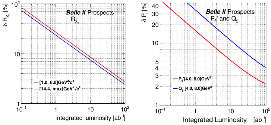
Figure 5: The Belle II sensitivity projection ?? for R_{X_s} (left) and P'_5 (and Q_5 ) (right) as a function of integrated luminosity.
