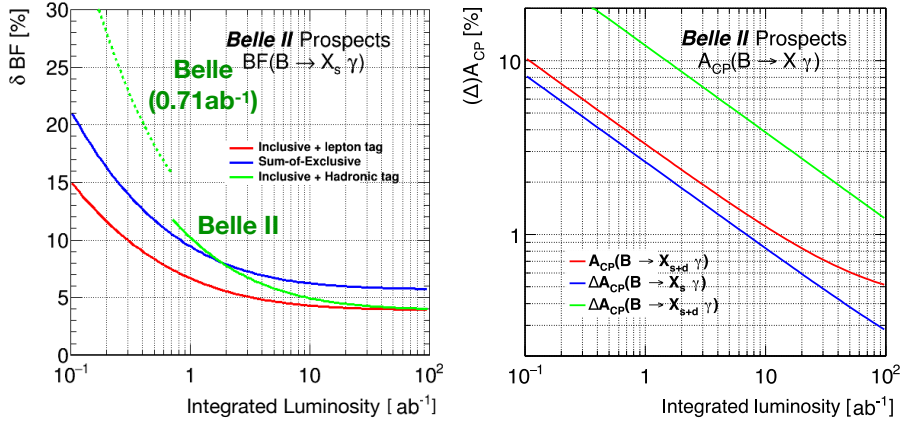
Figure 3: The Belle II sensitivity projection ?? for BF(B \rightarrow X_s \gamma) (left) and (\Delta)\mathcal{A}_{CP}(B \rightarrow X \gamma) (right) as a function of integrated luminosity. The green line in BF is discontinued assuming the improvement of hadronic tagging in the Belle II experiment.
