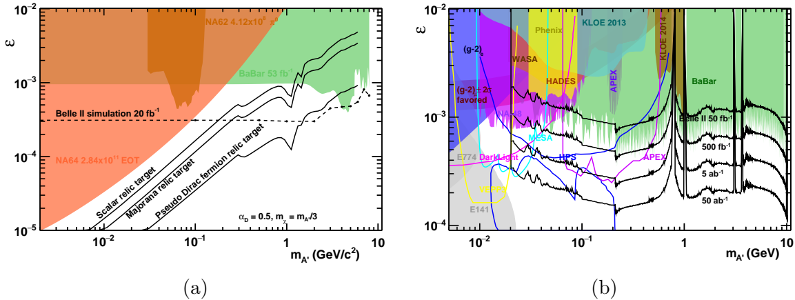
Figure 7: a) Expected sensitivity to the kinetic mixing strength for the process e^+e^- \rightarrow \gamma_{ISR} A' , A' \rightarrow \chi\bar{\chi} compared to other experiments [11]. b) Projected limits for Belle 2 on the dark photon kinetic mixing parameter \epsilon and mass m_{A'} via the visible decay process e^+e^- \rightarrow \gamma_{ISR} A' , A' \rightarrow \bar{l}l compared to other experiments [11].
