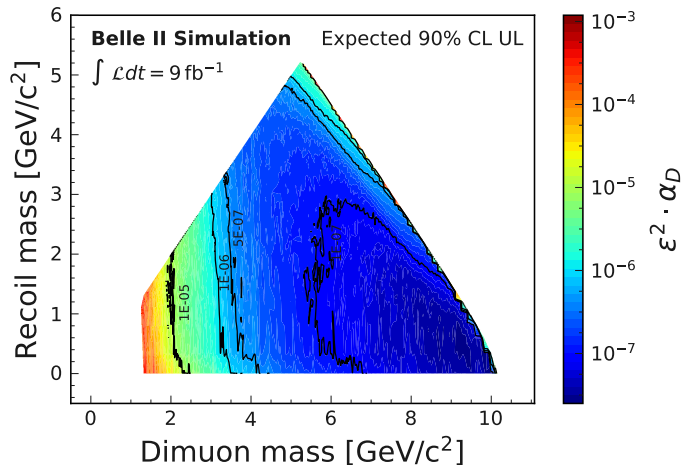
Figure 8: Expected upper limits (90% C.L.) to the coupling constant \epsilon^2 \cdot \alpha_D for the process e^+e^- \rightarrow A'h' , A' \rightarrow \mu^+\mu^- , h' \rightarrow \text{inv.} , with an integrated luminosity of 9\text{fb}^{-1} , corresponding, roughly, to the 2019 data-taking integrated luminosity.
