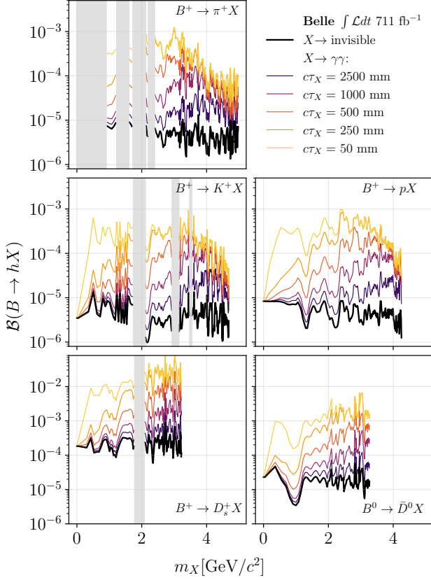
FIG. 2. Upper limits on the branching fraction \mathcal{B}(B \rightarrow hX_{\text{inv}}) at 90% CL as a function of m_{X_{\text{inv}}} are shown in black. Replacing the invisible decay assumption with X \rightarrow \gamma\gamma yields the colored limits, shown for several orders of magnitude of c\tau_X . Mass regions vetoed for known SM particles \pi^0 , K^{(*)0} , D^{(*)0} , \eta_c , \chi_{c1} , and \psi(2S) are shaded gray. Not all veto regions apply to every channel.
