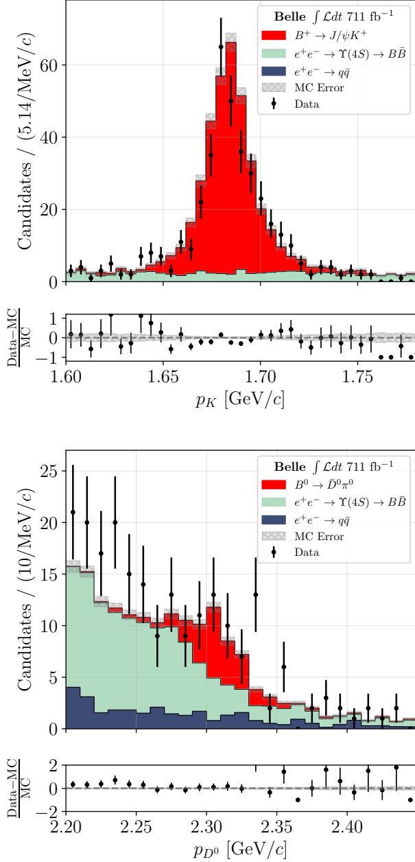
FIG. 1. Momentum distributions of the K^+ and D^0 in the B_{\text{sig}} -frame for the two control channels, B^+ \rightarrow J/\psi K^+ (top) and B^0 \rightarrow \bar{D}^0 \pi^0 (bottom), respectively, overlaid with the expected distributions from simulation.
