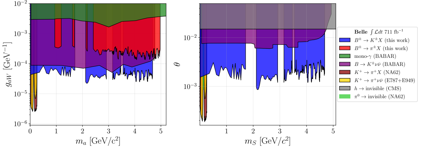
FIG. 3. Excluded regions for m_{X_{inv}} up to 5.1 GeV/c 2 at 90% CL shown for: (a) the coupling g_{aW} in the invisible ALP scenario from Ref. [22], and (b) the mixing angle \theta for the dark scalar in the missing energy scenario from Ref. [37]. Exclusions from BABAR [44, 83], NA62 [18, 20], E949 [21], and CMS [84] are overlaid for comparison.
