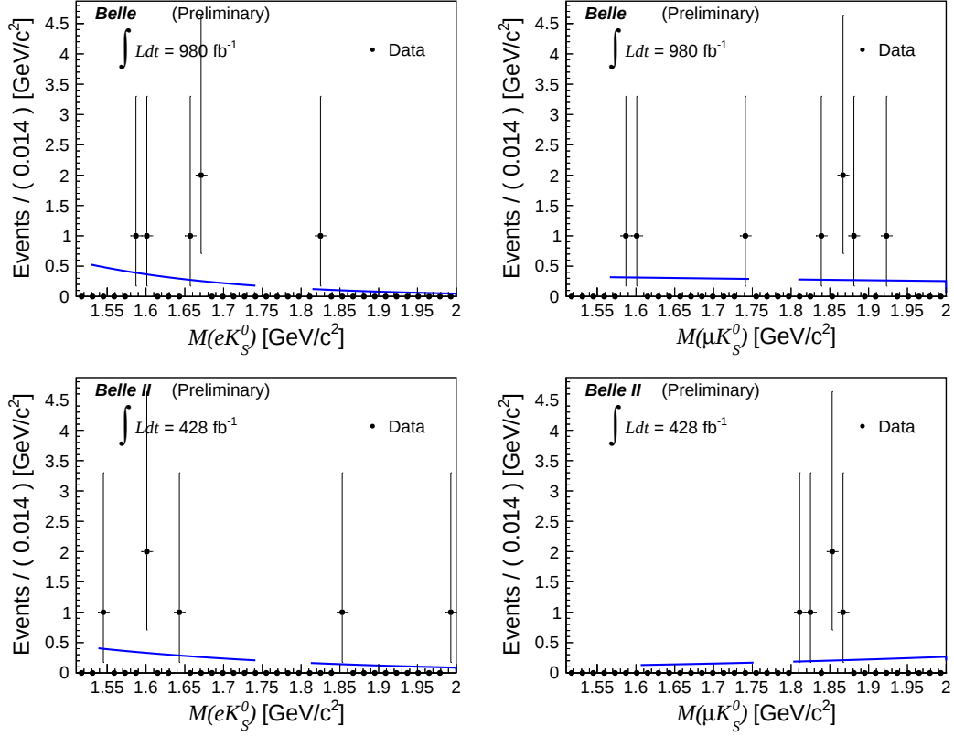
Figure 5. Fits (blue solid line) to selected events (points with error bars) in the RSB region as function of M(\ell K_S^0) . Top row shows the electron (left) and muon (right) channels for Belle, the bottom row shows the electron (left) and muon (right) channels for Belle II.
