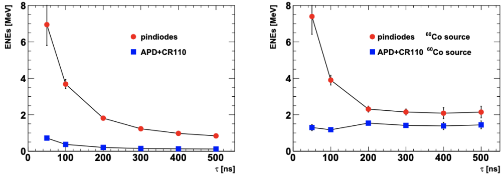
Figure 9.7: Equivalent Noise Energy as a function of the shaping time comparing pin diodes with APD with CR110 amplifier without (left) and with (right) 60 Co source.
