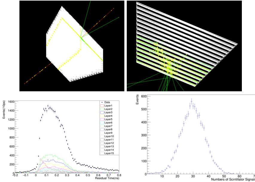
Figure 6.9: Geant4 simulation results for one barrel octant of an upgraded KLM with precision time-of-flight scintillators. Top left: response for one 1 GeV/ c muon. top right: response for one 1 GeV/ c K_L meson. Bottom left: time distribution of hits in each layer and cumulative for the K_L cluster; the resolution of (95 \pm 4) ps is extracted from a fit to the leading-edge (earliest) times in this graph. Bottom right: population distribution of scintillator signals for the K_L cluster.
