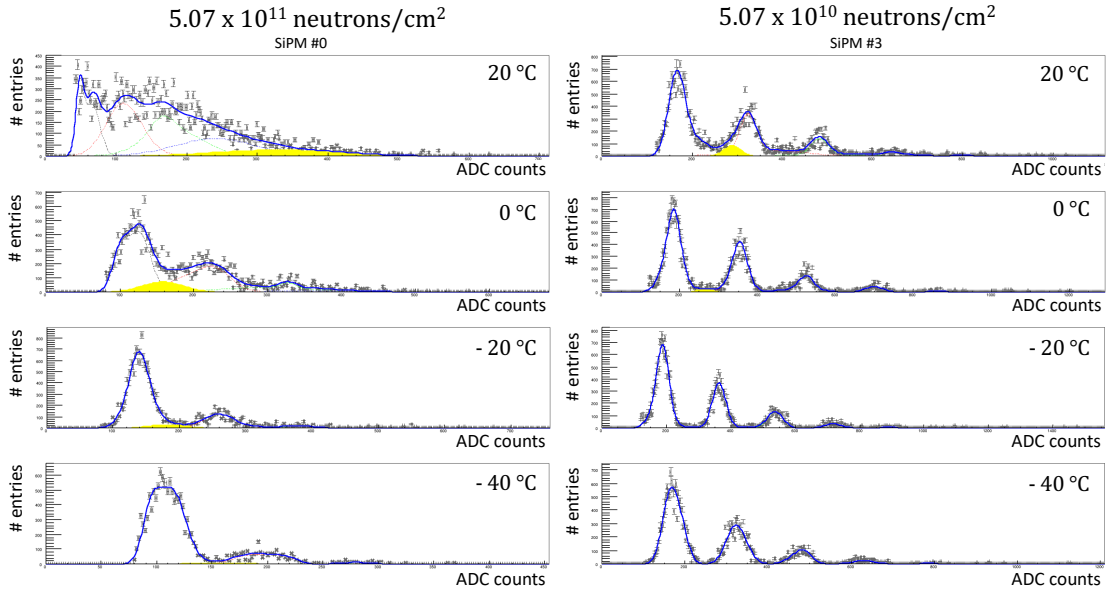
Figure 6.5: Single photoelectron spectrum (number of entries vs signal amplitude in ADC counts) for an irradiation of 5.07 \times 10^{11} \text{ n}/\text{cm}^2 (left) and 5.07 \times 10^{10} \text{ n}/\text{cm}^2 (right) at different temperatures. Signal peaks have been fitted with the convolution of a Poisson distribution with some double Gaussian functions (dashed lines), a Gaussian background (yellow) has been added to the fit.
