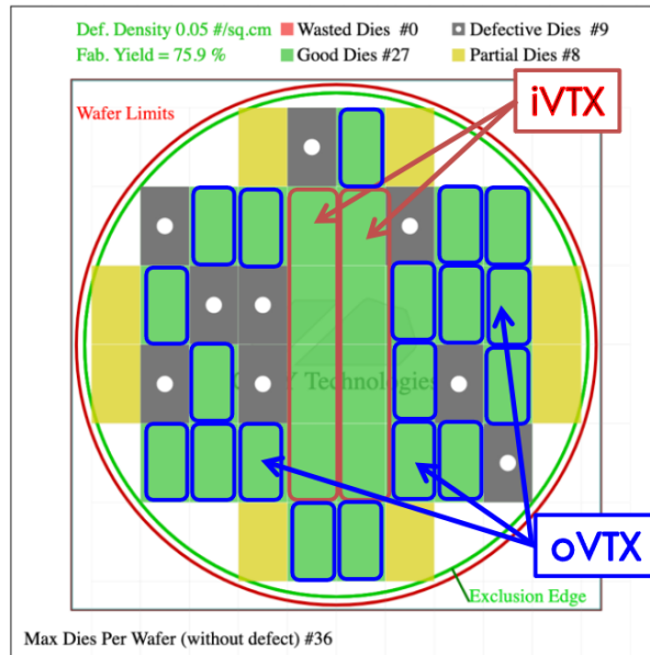
Figure 5.1: Sketch of the OBELIX reticle occupancy over an 8 inch diameter wafer. Red rectangles indicate possible dicing area including 4 consecutive sensors for iVTX ladders, while blue rectangles stand for individual chip dicing for oVTX stave population.
