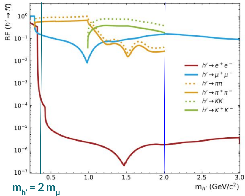
BR of the dark Higgs decaying into four different final states as a function of its mass.
