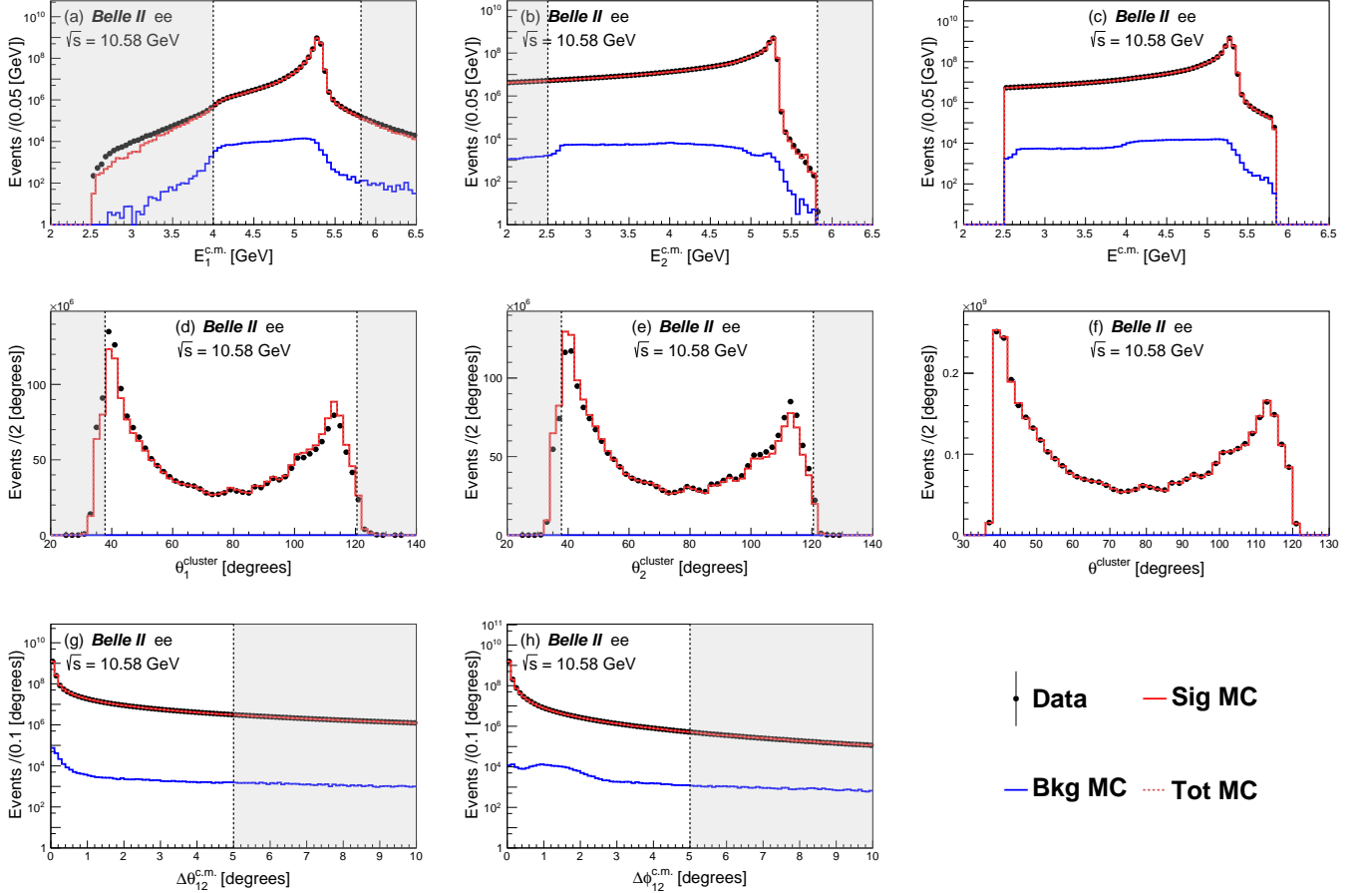
Figure 1: Kinematic distributions of Bhabha signal candidates in data and MC. The first row contains distributions of the c.m. energy of the higher-energy final-state particle (a), the lower-energy final-state particle (b), and each of the two final-state particles (c). The second row represents distributions of polar angle of ECL clusters of the higher-energy final-state particle (d), the lower-energy particle (e), and each of the two final-state particles (f) in the lab frame. Subfigure (g) shows the distribution of the polar opening angle ( \Delta\theta_{12}^{c.m.} = |\theta_1^{c.m.} + \theta_2^{c.m.} - 180^\circ| ), while subfigure (h) shows the distribution of the azimuthal opening angle ( \Delta\phi_{12}^{c.m.} = ||\phi_1^{c.m.} - \phi_2^{c.m.}| - 180^\circ| ). Each subfigure shows one parameter from the event selection criteria where all other criteria have been applied except for that shown in the figure. All the criteria are applied in subfigures (c) and (f). “Data” in the legend signifies the collision data from the \Upsilon(4S) dataset, while “Sig MC”, “Bkg MC”, and “Tot MC” correspond to the signal (MC Bhabha events), background (MC samples except for signal events), and total MC samples (the sum of both the signal and background samples), respectively. The error bars are invisible due to the large size of the sample. The dashed histogram for “Tot MC” overlaps with the solid histogram of “Sig MC”, making the “Tot MC” histogram invisible. The vertical black dashed lines represent the selection criteria for signal events. Events in the shaded regions are removed by the selection criteria.
