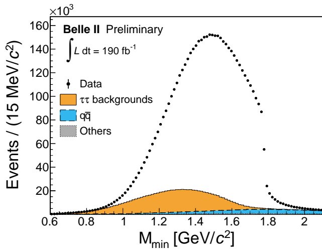
Figure 1: Spectrum of M_{\min} in experimental data (dots), along with simulated background contributions from e^+e^- \rightarrow \tau^+\tau^- events with decays other than \tau^- \rightarrow \pi^-\pi^+\pi^-\nu_\tau (orange area with solid line), e^+e^- \rightarrow q\bar{q} events (blue area with dashed line), and other background sources (gray area with dotted line).
