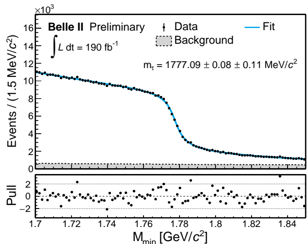
Figure 3: Top: Spectrum of M_{\min} in experimental data (dots) with fit result (solid blue line) and background contribution (gray-filled area) overlaid. Bottom: Differences between data and fit result divided by the statistical uncertainties.
