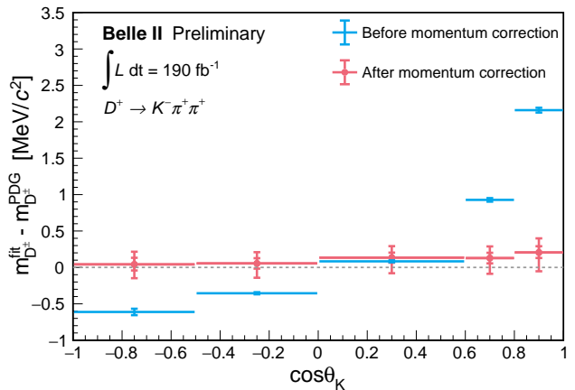
Figure 4: Deviation of the D^\pm invariant-mass peak position from the known value before (blue) and after (red) momentum corrections as a function of the cosine of the kaon polar angle \theta_K . The vertical error bars on the blue points indicate the statistical uncertainties in determining the peak position while the vertical error bars on the red points indicate the statistical and total uncertainties of the applied momentum corrections.
