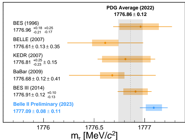
Figure 5: Summary of the most precise \tau -mass measurements [5–9] compared with the result of this work. The vertical gray band indicates the average value of previous measurements [32]. The inner bars represent the statistical uncertainties, while the outer bars indicate the total uncertainties.
