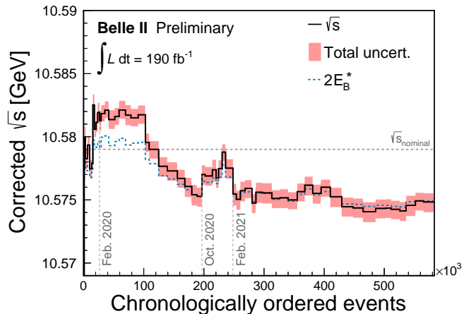
Figure 2: Corrected center-of-mass energy \sqrt{s} (solid) and center-of-mass energy of B\bar{B} pair 2E_B^* (dashed blue line) as functions of data-taking time, expressed in terms of chronologically ordered event numbers. The horizontal dashed line represents the nominal center-of-mass energy, \sqrt{s}_{\text{nominal}} = 10.579 GeV, and the vertical dashed lines indicate the start of different data-taking periods. The 68.3% confidence level band of \sqrt{s} is displayed as shaded area.
