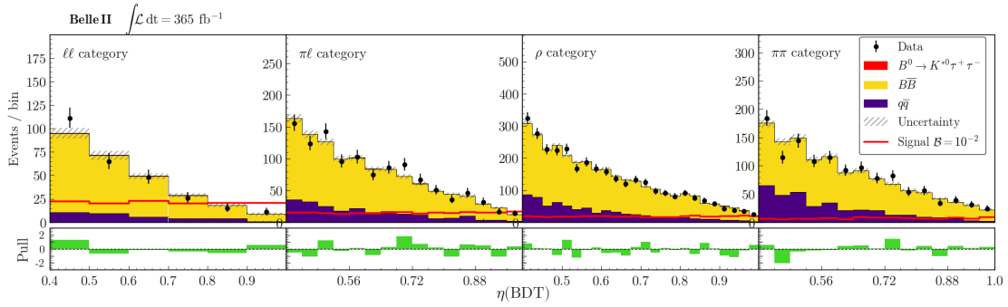
Figure 2: Distributions of \eta(\text{BDT}) in the SR for the four signal categories. The fit results are shown for the two background components ( B\bar{B} and q\bar{q} ) and the B^0 \rightarrow K^{*0}\tau^+\tau^- signal, with a fitted branching fraction of [-0.15 \pm 1.01] \times 10^{-3} . A B^0 \rightarrow K^{*0}\tau^+\tau^- signal distribution, scaled assuming a branching fraction of 10^{-2} , is shown as reference. The bottom panel shows the pull distributions. The histograms for the four categories are available on HEPData [37].
