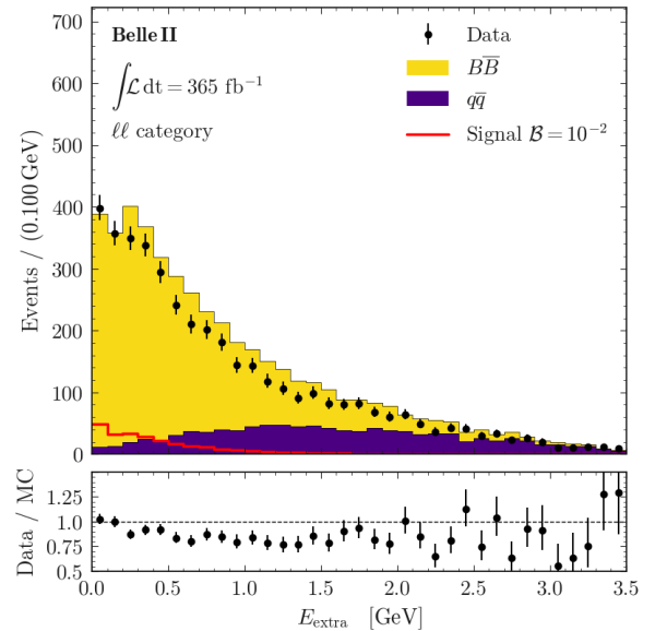
Figure 1: Distribution of E_{\text{extra}} for events passing the nominal selection, with all the corrections applied, for the \ell\ell signal category. The signal B^0 \rightarrow K^{*0} \tau^+ \tau^- histogram is shown scaled assuming a branching fraction of 10^{-2} .
