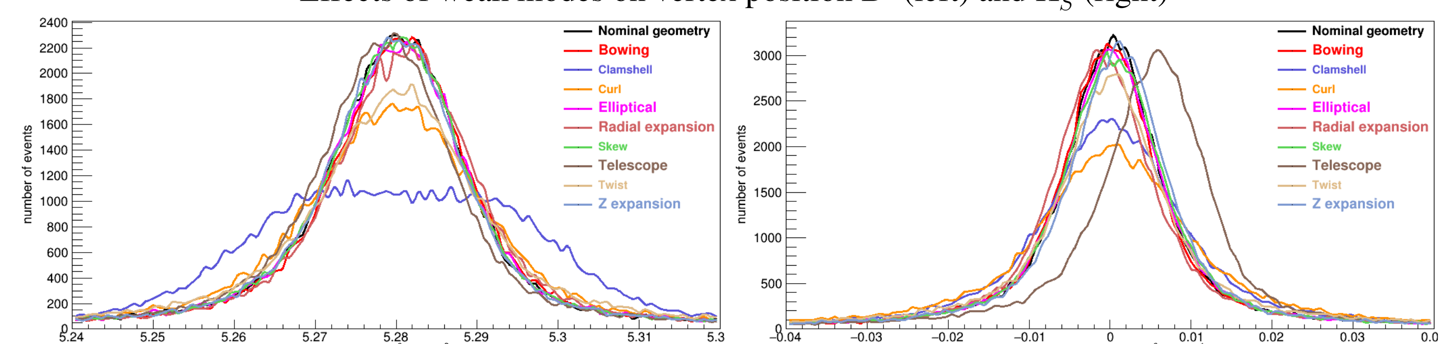
Effects of weak modes on mass (left) and momentum (right) of B^0 .
