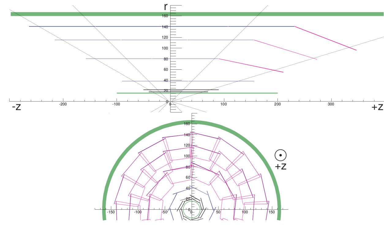
Cross-section of VXD in r-z (top) and r- \phi (bottom) plane. VXD consists of PXD (black), SVD trapezoidal wedged (pink) and SVD rectangular (blue) sensors. Dimensions are in millimeters.
