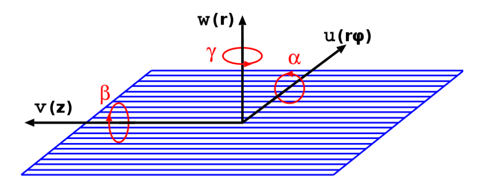
Alignment parameters of a planar sensor
