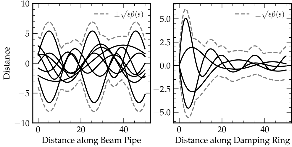
Figure 2.3: Sketch of betatron oscillations drawn with continuous lines and the corresponding beam envelope drawn with dashed lines. The emittance and the beam envelope are decreased in a damping illustrated on the right.
