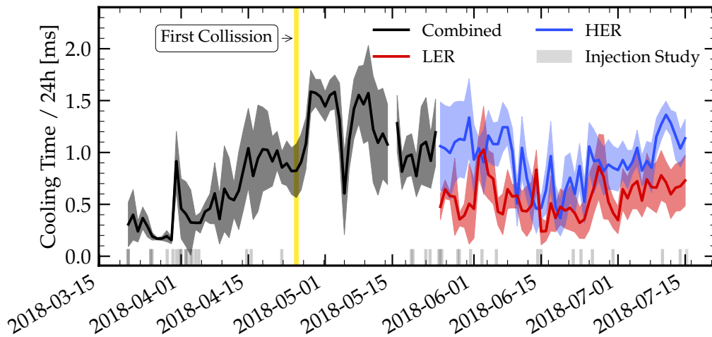
Figure 8.6: SuperKEKB cooling time in Phase 2. The cooling time is defined as time until 66% of the particle content has been observed in the waveform. The graphs represent the Mean90 \pm StdDev90 of the corresponding data source per day.
