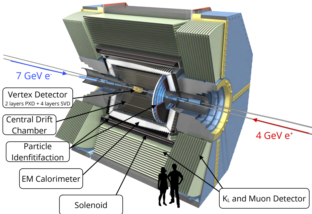
Figure 3.1: The Belle 2 detector. The sub-detector components are displayed correspondingly.
