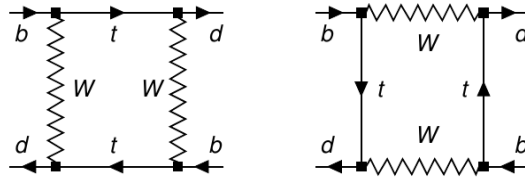
Figure 1.2: Dominant contributions to B\bar{B} -mixing in the Standard Model. Taken from [15].
