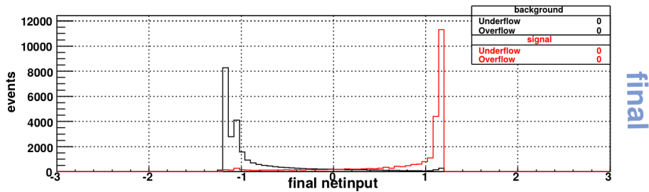
(d) Input into neural network after preprocessing.
