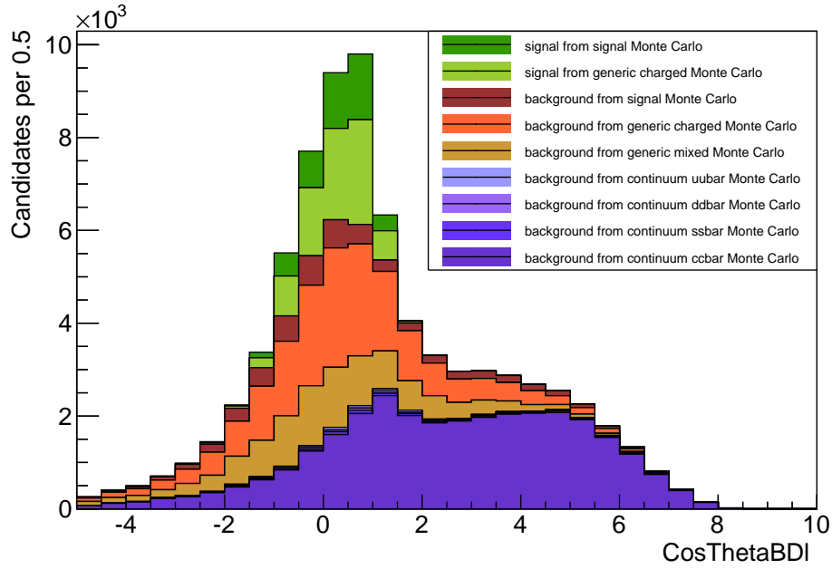
(b) Semileptonic candidates: \cos \Theta_{BDl} distribution with a purity of 32 % and a tagging efficiency of 0.35 %.
