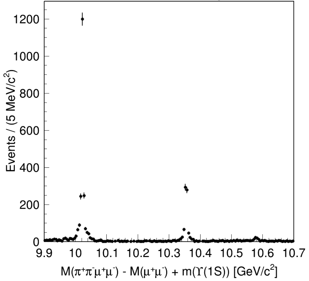
FIG. 2: Plot of M(\pi^+\pi^-\mu^+\mu^-) - M(\mu^+\mu^-) + m(\Upsilon(1S)) with a requirement of |M(\mu\mu) - m(\Upsilon(1S))| < 75 \text{ MeV}/c^2 , where m(\Upsilon(1S)) represents the nominal \Upsilon(1S) mass.
