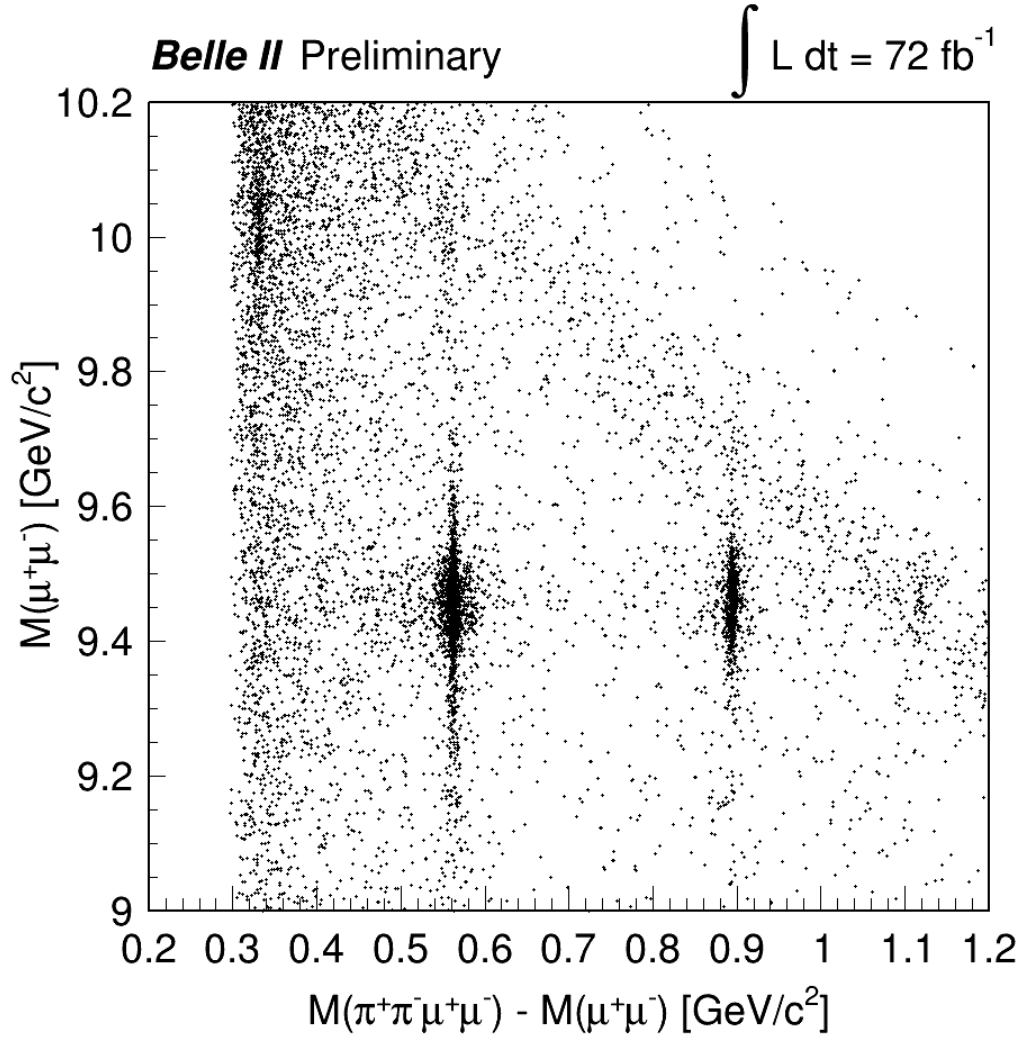
FIG. 1: Plot of M(\mu\mu) versus M(\pi^+\pi^-\mu^+\mu^-) - M(\mu^+\mu^-) for \Upsilon \rightarrow \mu^+\mu^- dipion decays. The clusters of points represent signal transitions.
