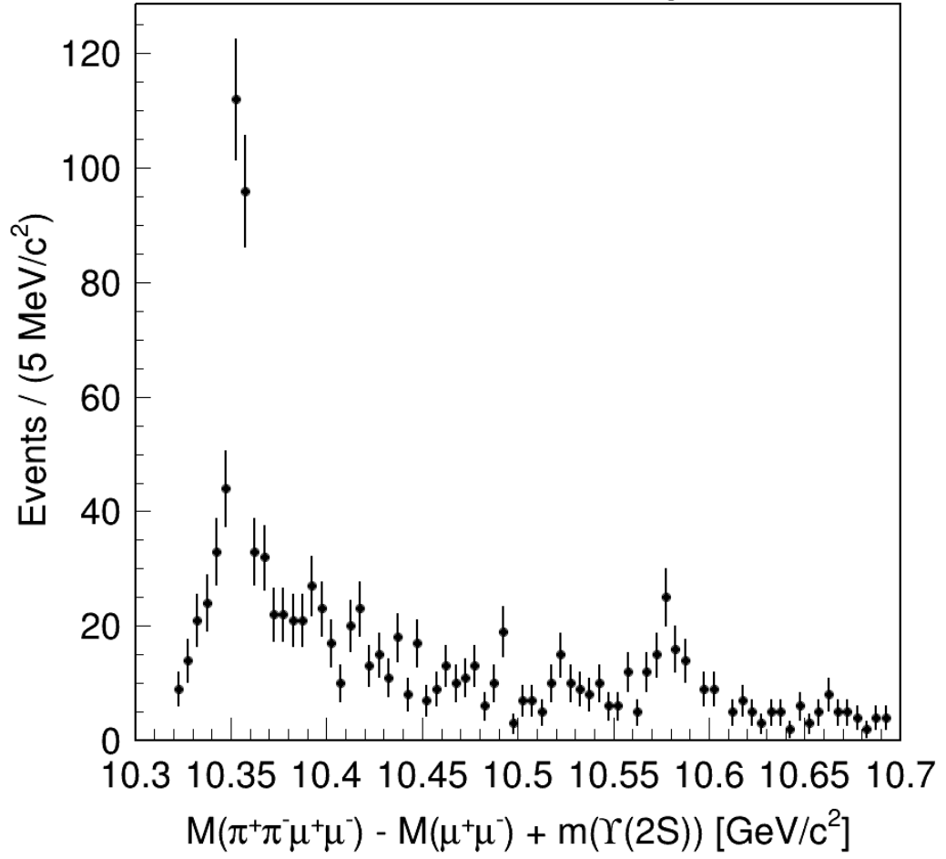
FIG. 3: Plot of M(\pi^+\pi^-\mu^+\mu^-) - M(\mu^+\mu^-) + m(\Upsilon(2S)) with a requirement of |M(\mu\mu) - m(\Upsilon(2S))| < 75 \text{ MeV}/c^2 , where m(\Upsilon(2S)) represents the nominal \Upsilon(2S) mass.
