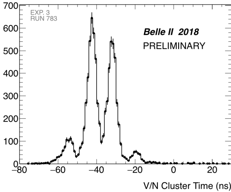
Figure 2: This figure shows the reconstructed time of the N-side clusters of the Large Rectangular Sensor. Only clusters associated to tracks have been selected, no selection on the tracks is applied. We have used data from Experiment 3 Run 783. The internal document reference is BELLE2-NOTE-TE-2018-005.
