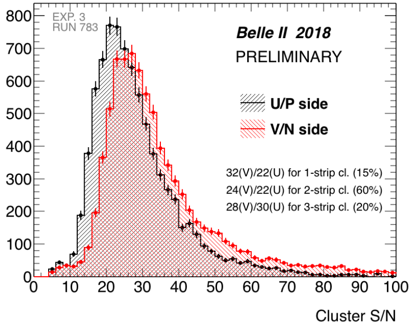
Figure 1: This figure shows the signal-over-noise ratio (SNR) of P and N clusters for the Large Rectangular Sensor. Only clusters associated to tracks have been selected, no selection on the tracks is applied. We have used data from Experiment 3 Run 783. The internal document reference is BELLE2-NOTE-TE-2018-005.
